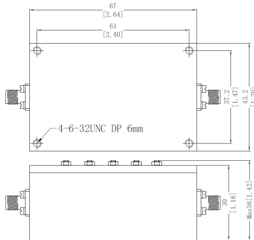
Physical Dimensions ( \pm 0.3\text{mm} )
